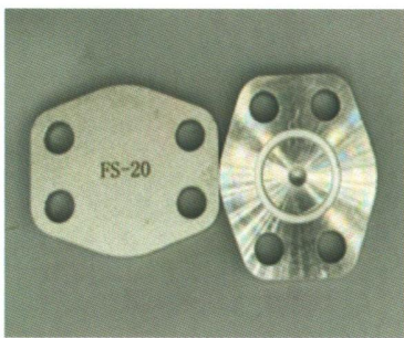
4FL/4FS 堵板 L/S SERIES FLANGE O-RING PLUG
