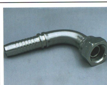
22192 90° BSP FEMALE MULTISEAL
