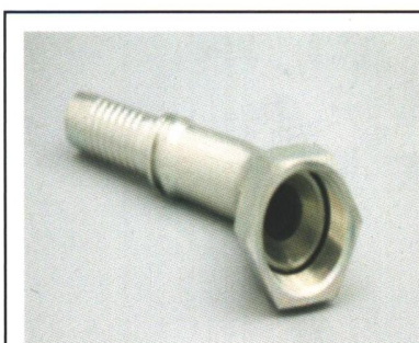
28642 Model: FEMALE 60° CONE
