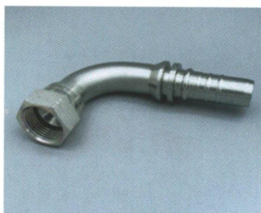
26793 90° JIC FEMALE 74° CONE SEAT
